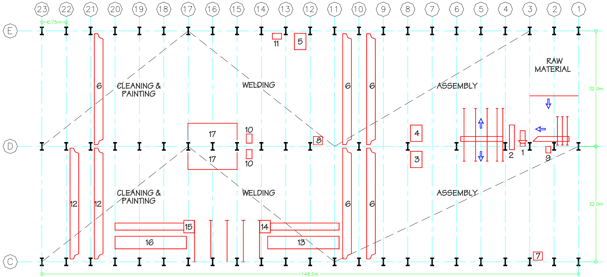
FACTORY MACHINERY LAYOUT
